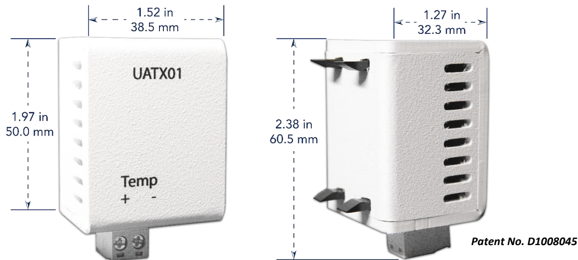
Figure 1 - Temperature Sensor with Dimensions
